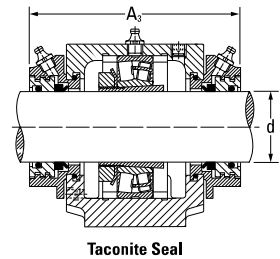
Taconite Seal
