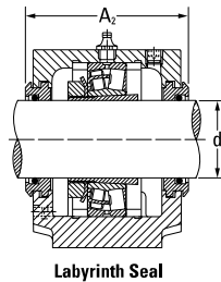
Labyrinth Seal
