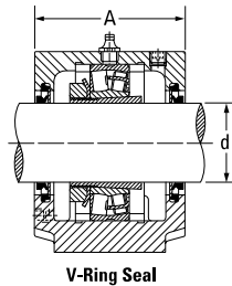
V-Ring Seal
