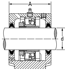
Double-Lip Seal
