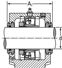
Labyrinth Seal
