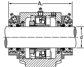
Taconite Seal
