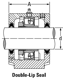
Double-Lip Seal
