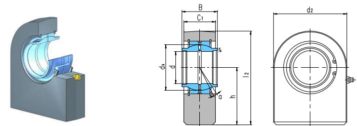
Sliding contact surfaces: Steel / Steel
